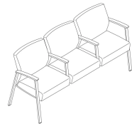
Open Arm Spanner W69.5" D23.5" H33.81" Seat: W66" D17.5" H19" Arm Height: 27.5"
