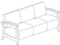
Open Arm Sofa W70.5" D30" H33" Seat: W66" D19.5" H19" Arm Height: 27"
