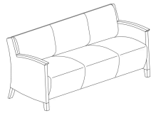
Closed Arm Sofa W70.5" D30" H33" Seat: W66" D19.5" H19" Arm Height: 27"
