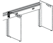
End Beam W 20.25, 26.25, 32.25, 38.25, 44.25, 50.25, 56.25, 62.25, 68.25, 74.25, 80.25" D 3.5" H 5.75"
