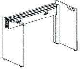
Standalone Beam W 36, 42, 48, 54, 60, 66, 72, 78" D 3.5" H 5.75"
