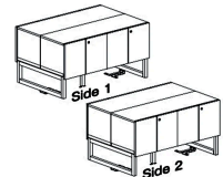
Dual-Sided Panel Supported W 42, 48, 54, 60, 66, 72" D 29.25" H 25"
