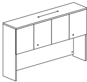
Overhead with 4 Laminate Doors W 60, 66, 72" D 16" H 43"
