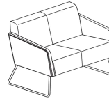
Loveseat W45.75" D30.25" H31.5" Seat: W38" D20.25" H18.5" Arms: H26.25"
