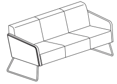
Sofa W72.5" D30.25" H31.5" Seat: W63.5" D20.25" H18.5" Arms: H26.25"
